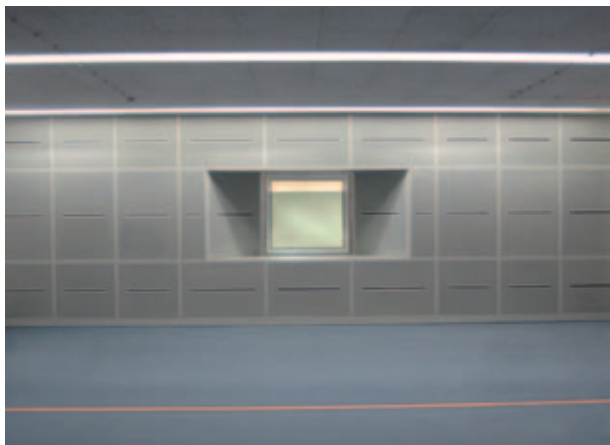
Air distribution wall with perforated discharge panels and linear slot diffusers Window for the supervision of the shooter with air distributing embrasures
